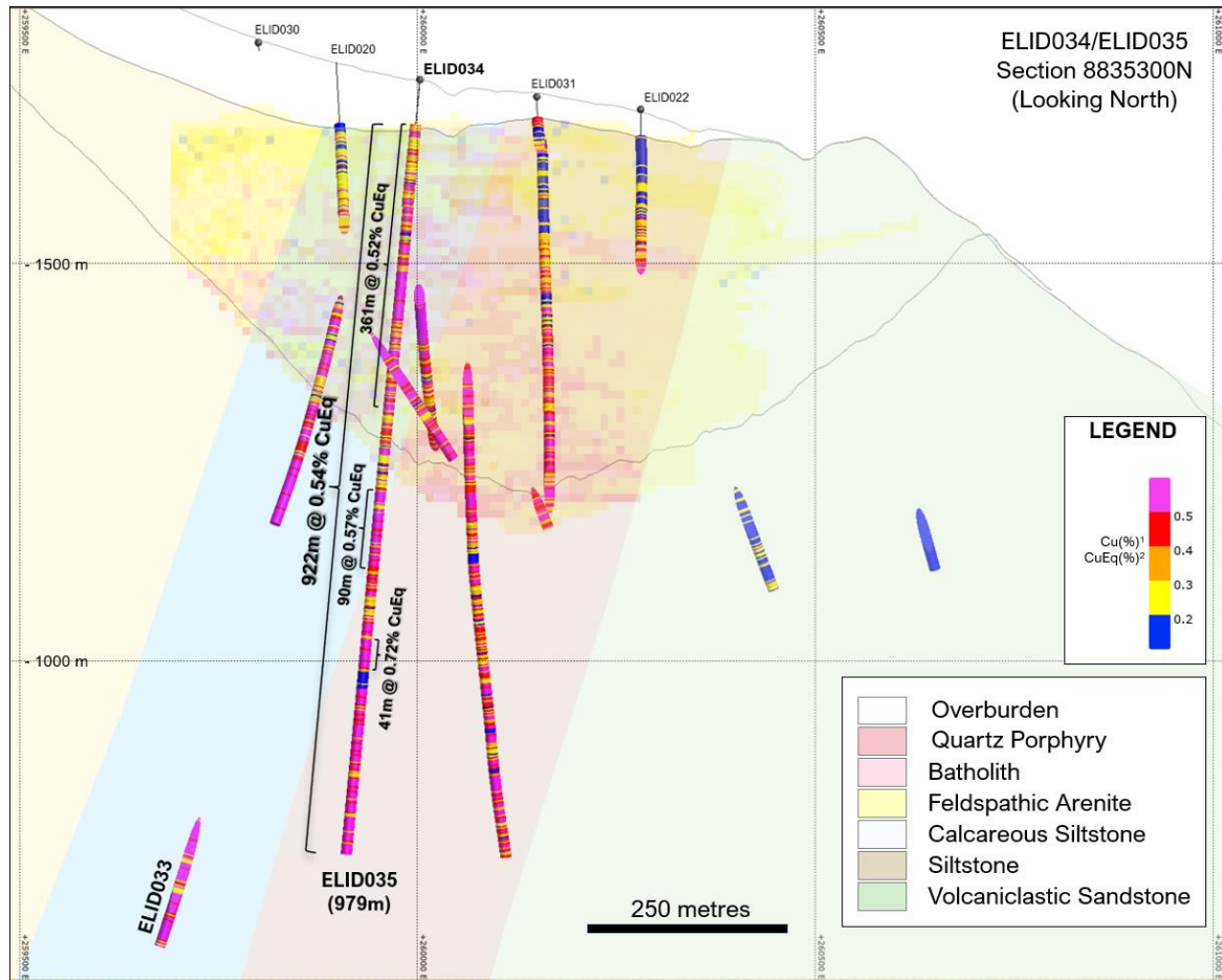
Figure 3: An east-west oriented geological cross section along northing 8835300N containing drill holes ELID034 and ELID035. The section shows the CuEq 2 geochemical assay results along the drill hole traces as well as length-weighted assay intervals of CuEq 2 geochemistry for ELID035.
