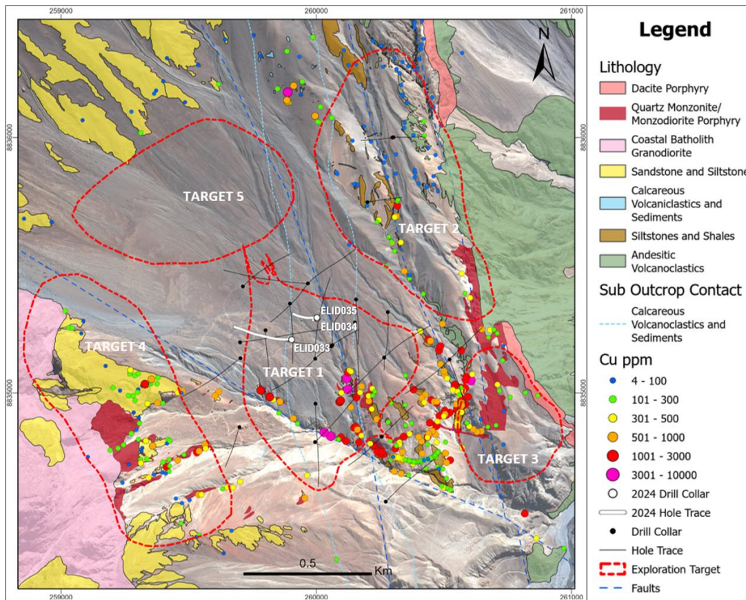
Figure 1: Plan map showing the location of the completed drill holes from the Phase-III diamond drill program at Elida.
