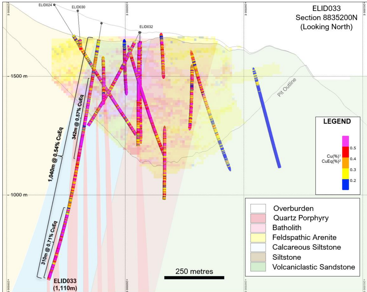
Figure 2: An east-west oriented geological cross section along northing 8835200N containing drill hole ELID033. The section shows the CuEq 2 geochemical assay results along the drill hole traces as well as length-weighted assay intervals of CuEq 2 geochemistry for ELID033.
