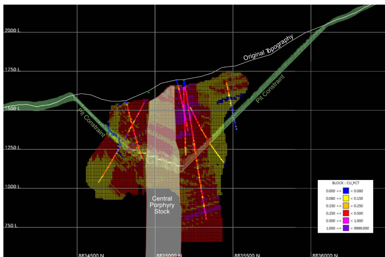
Figure 6. Section through 260050 E to illustrate the position of the constraining pit shell in relation to the original topographic surface and the block model used for the Mineral Resource estimate. The shaded area is the interpreted position of the low-grade quartz monzonite porphyry stock that occupies the core of Zone. Please refer to Figure 1 for the section location.
