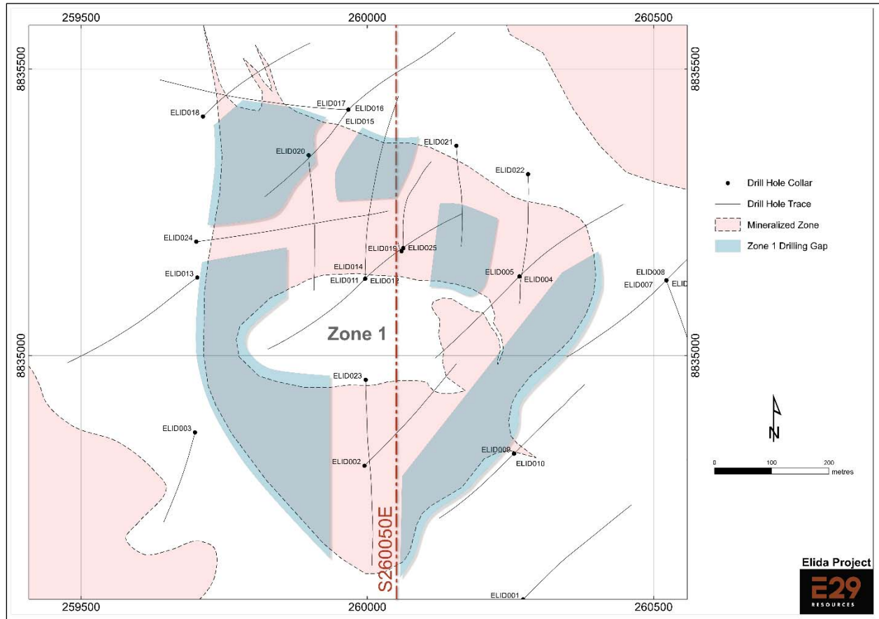
Figure 7. Details of Elida Zone 1, showing areas identified for follow-up drilling, which will be designed to better resolve Cu and molybdenite grade distribution near surface and within the constraining pit shell and more accurately define limits of mineralization particularly on the northwest and southwest edges of Zone 1.
