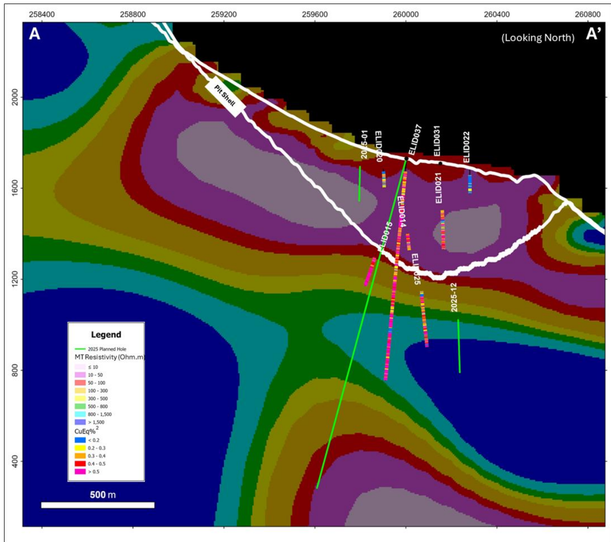
Figure 2: A 2D section (looking north) along drill hole ELID037 plotted over the 3D MT resistivity model, drill hole traces from previous programs showing CuEq² (%) grades, and the outline of the pit-shell. The location of this section (A-A') is provided in Figure 1.
